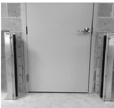
Stages of Set Up for Flood Logs. Color Coded For Easy Assembly
